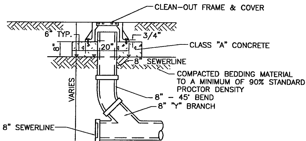
SIDE VIEW
