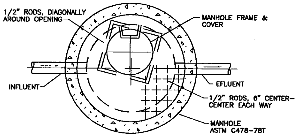
TOP VIEW
