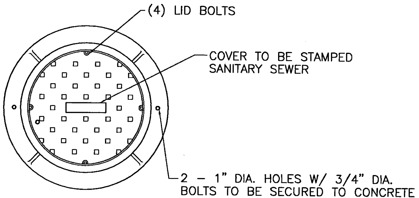
TOP VIEW
