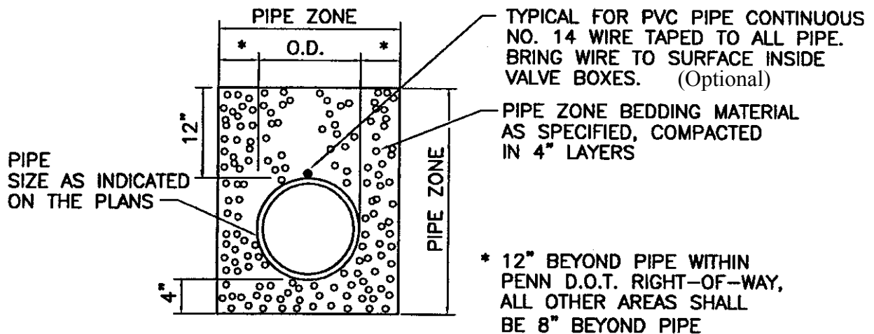
PVC PIPE
