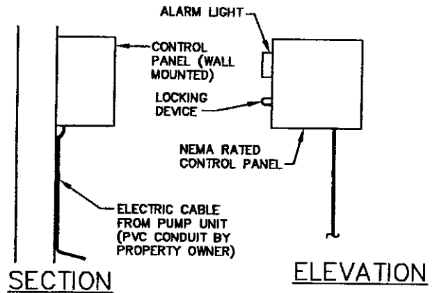
CONTROL PANEL
