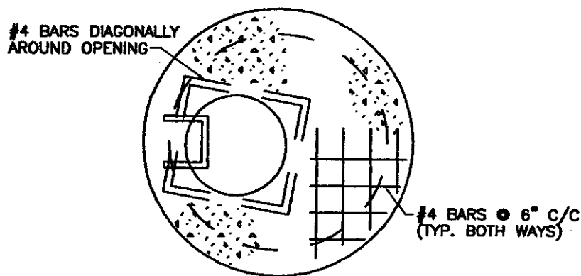
PLAN
