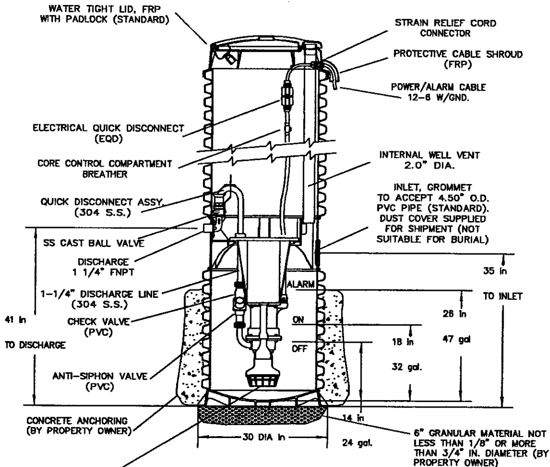
TYPICAL DETAIL
