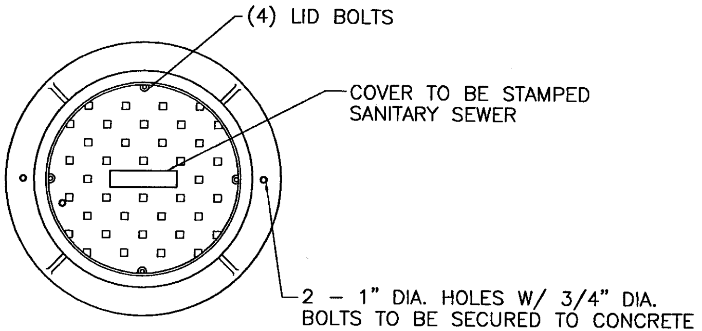
TOP VIEW
