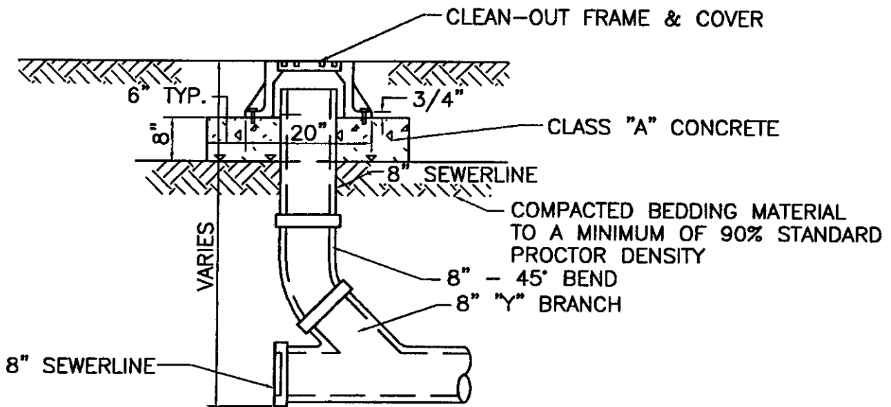
SIDE VIEW
